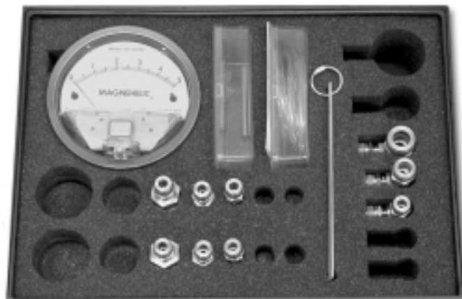
Internal purge pressure kit for 1/4, 3/8, and 1/2 in. tubing
